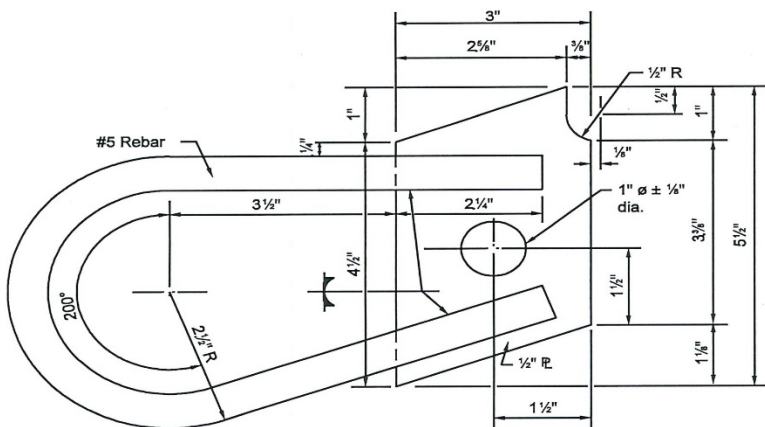
ANCHOR PLATE ALTERNATE A-1
