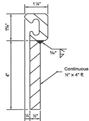
EXTRUSION & PLATE ASSEMBLY DETAIL
