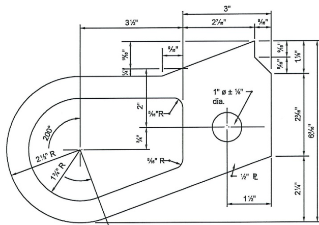
ANCHOR PLATE ALTERNATE B-2
